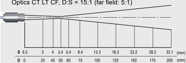
Optics CT LT CF, D:S = 15:1 (far field: 5:1)
